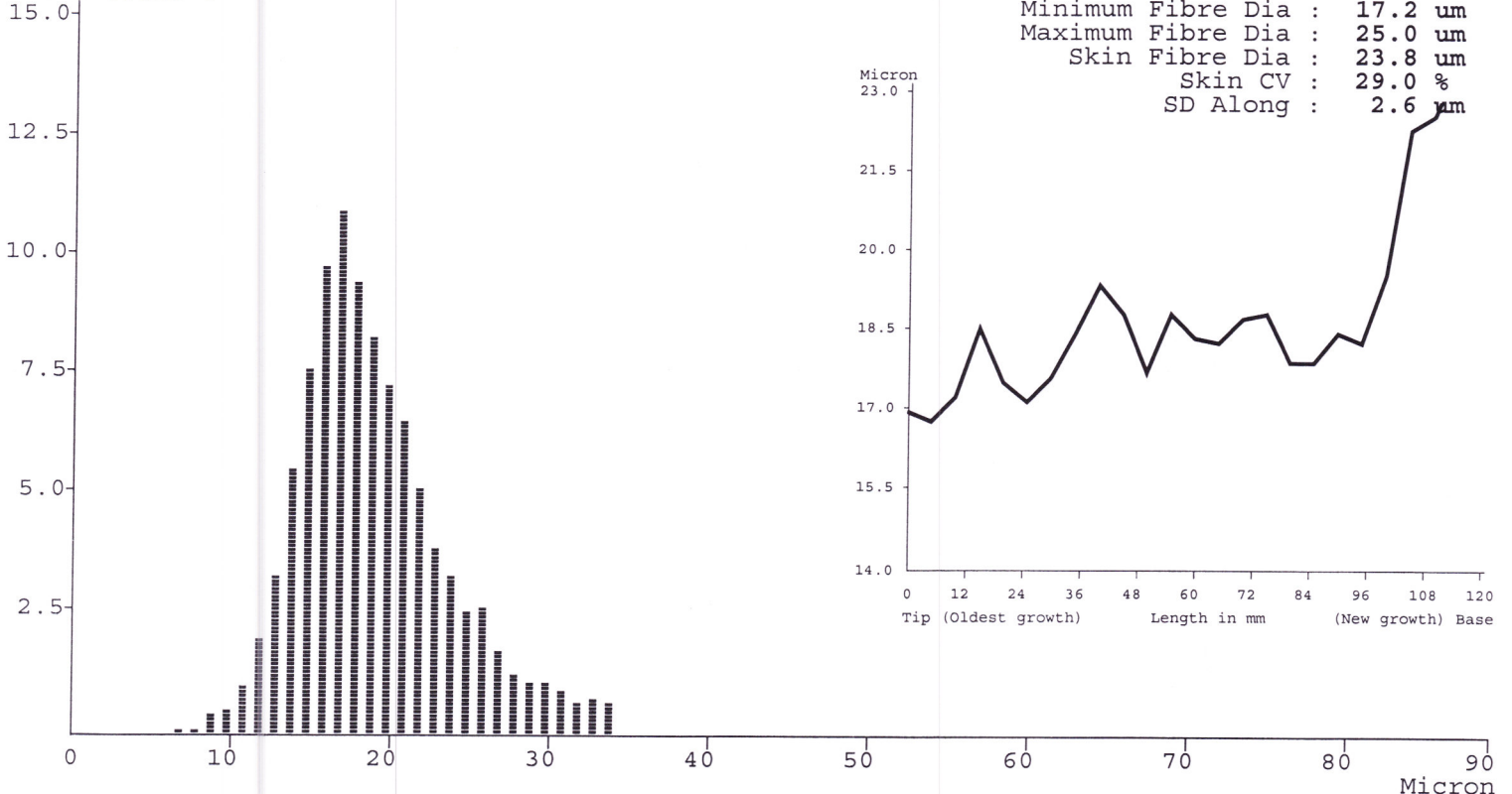
Fibre Count %
